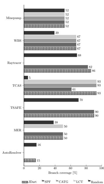
Fig. 8: Branch coverage.
