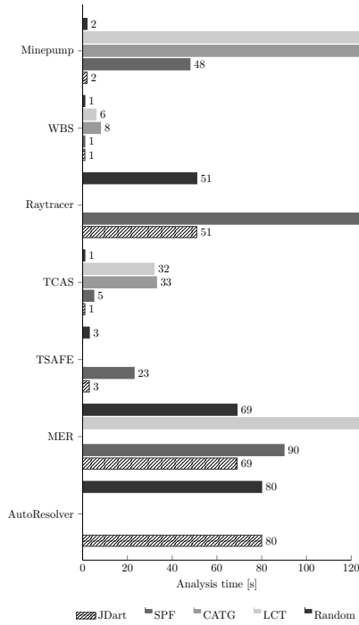
Fig. 6: Analysis time.
